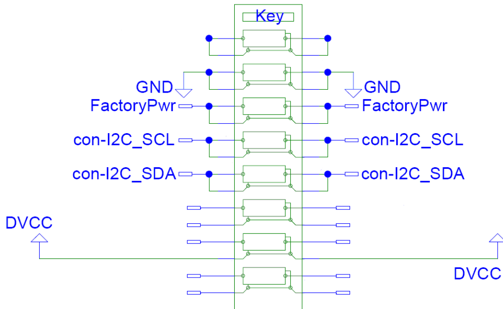
Figure 6 CO 2 Engine™ -BLG/ELG edge connector, (seen from component side)
